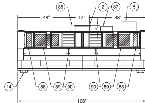
STADIUM ST-40-T FRONT VIEW
