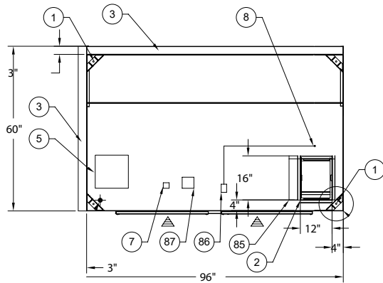
STADIUM ST-20-T TOP VIEW
