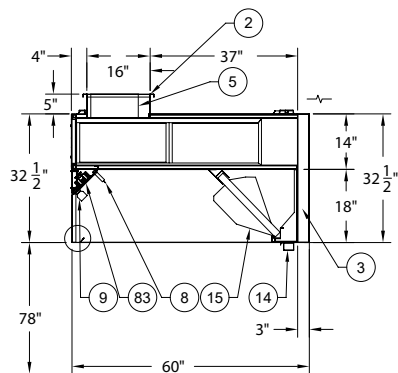
STADIUM ST-20-T SIDE VIEW
